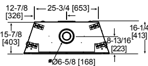
Top View Corner Installation
